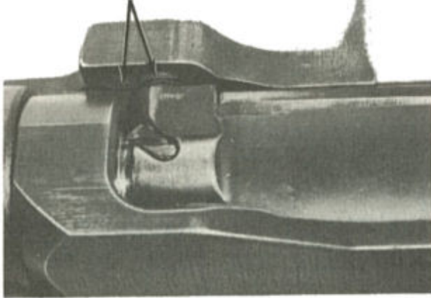
CAMMING SURFACES IN HUMP OF OPERATING ROD
